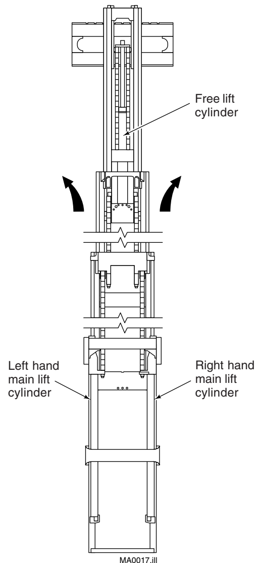
Figure 7. Extending upright viewed from driver seat.
